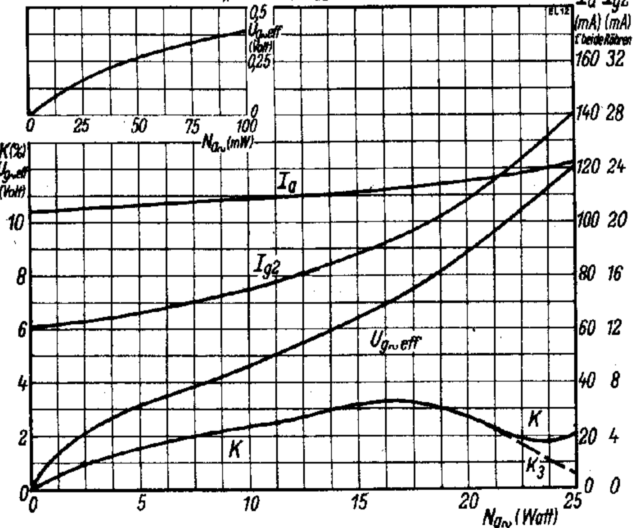
Kennlinienfeld 13 I_a, I_{g2}, U_{g,eff}, K = f(N_{a,eff}), R_{g2} = 700 \Omega, U_b = 375 \text{ Volt}
