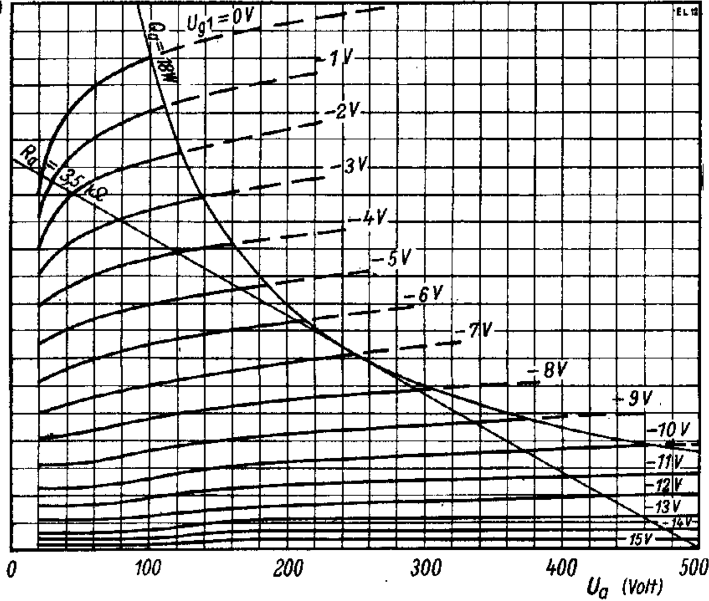
Kennlinienfeld 2 I_a = f(U_a) ; U_a = 250 Volt, U_{g1} = \text{Parameter}
