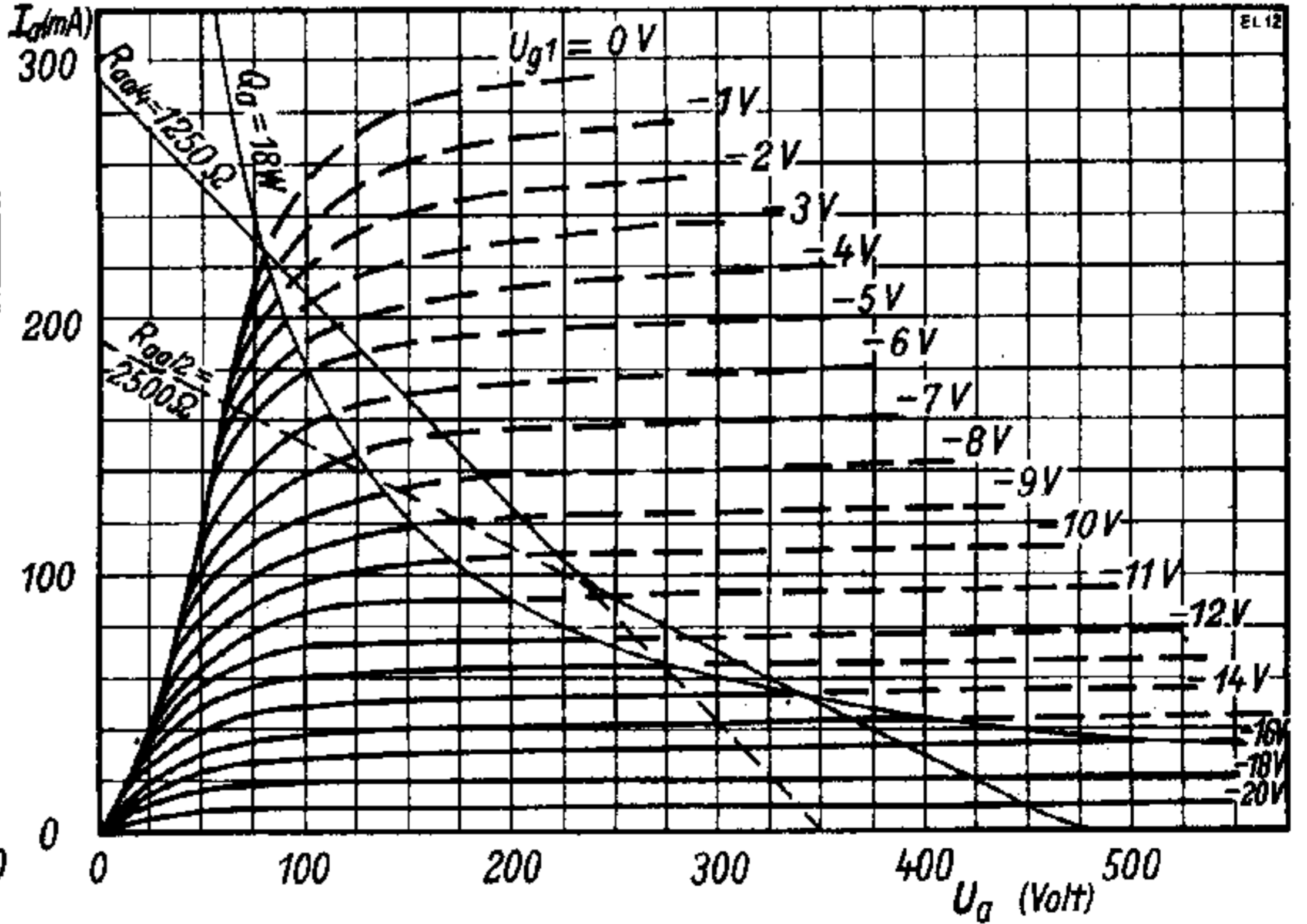
Kennlinienfeld 4 I_a = f(U_a) , U_{g2} = 350 Volt, U_{g1} = \text{Parameter}
