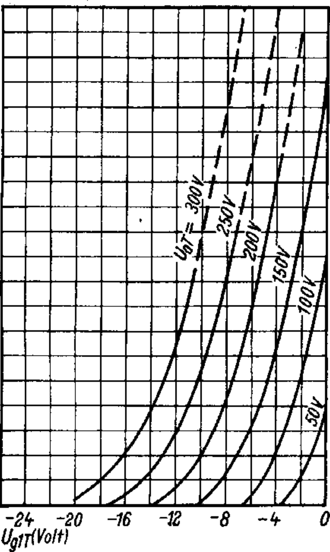
Kennlinienfeld 19 I_{aT} = f(U_{g1T}), U_{aT} = \text{Parameter}
