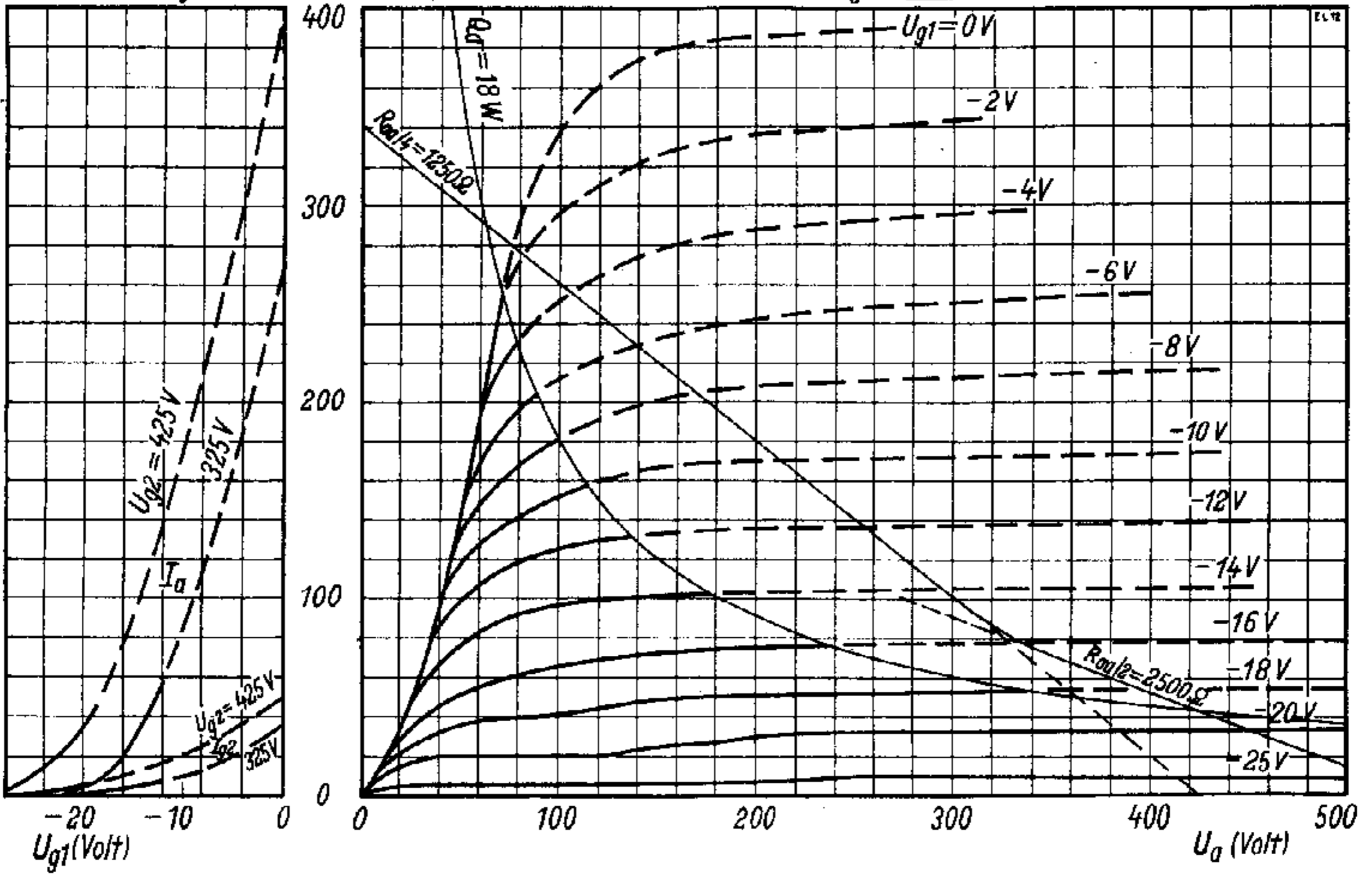
Kennlinienfeld 14 I_a, I_{g2} = f(U_{g1}) U_{g2} = \text{Parameter}, U_a = U_{g2} - 25 \text{ V}
