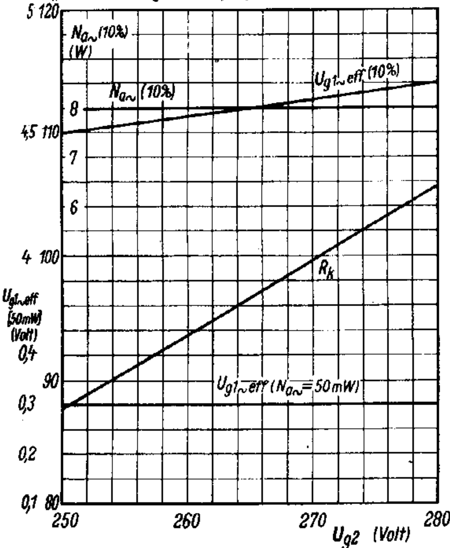
Kennlinienfeld 5 R_k, N_{a \sim}, U_{g1 \sim eff} = f(U_{g2}) U_a = 250 Volt, I_a = 72 mA
