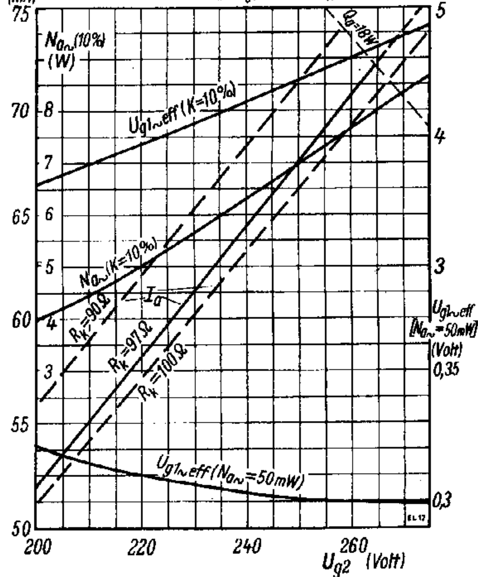
Kennlinienfeld 6 I_a, N_{a \sim}, U_{g1 \sim eff} = f(U_{g2}) U_a = U_{g2} - 15 Volt; R_k = 97 \Omega
